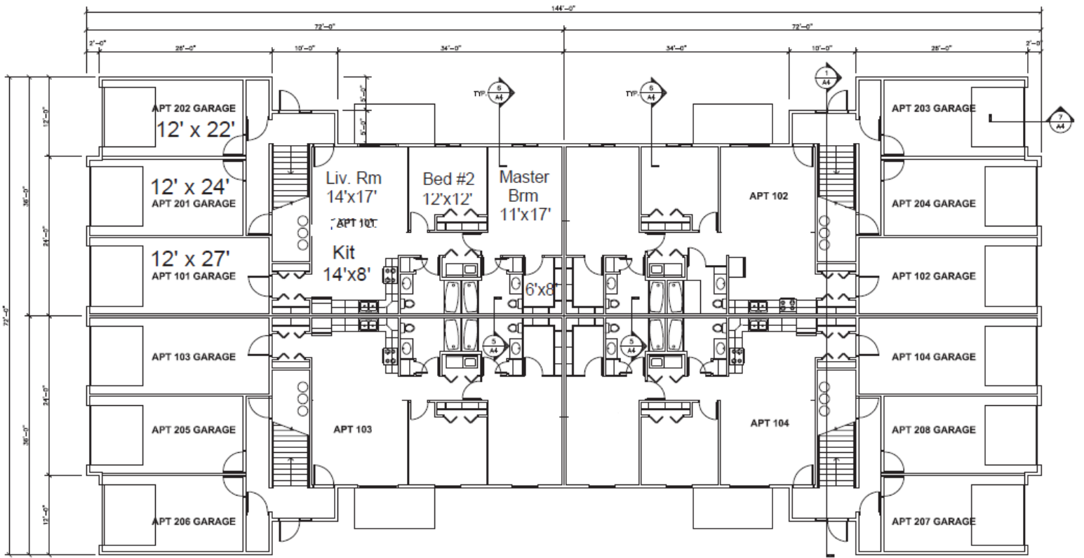
FIRST FLOOR PLAN 1/8" = 1'-0"
